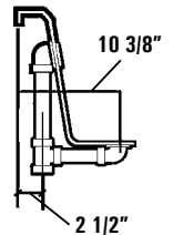
Rough-In Plumbing Measurements
